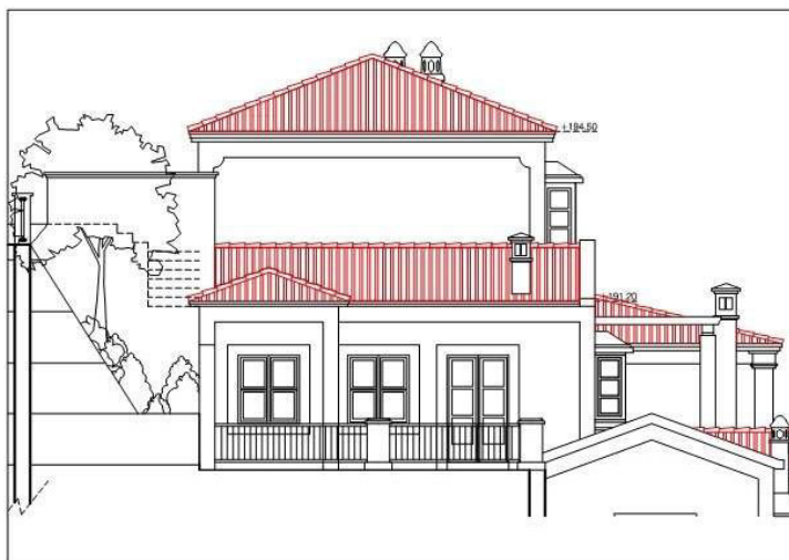
WEST ELEVATION
