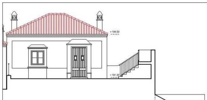
NORTH ELEVATION
