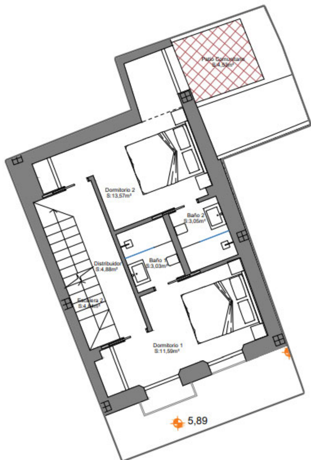
Middle floor
