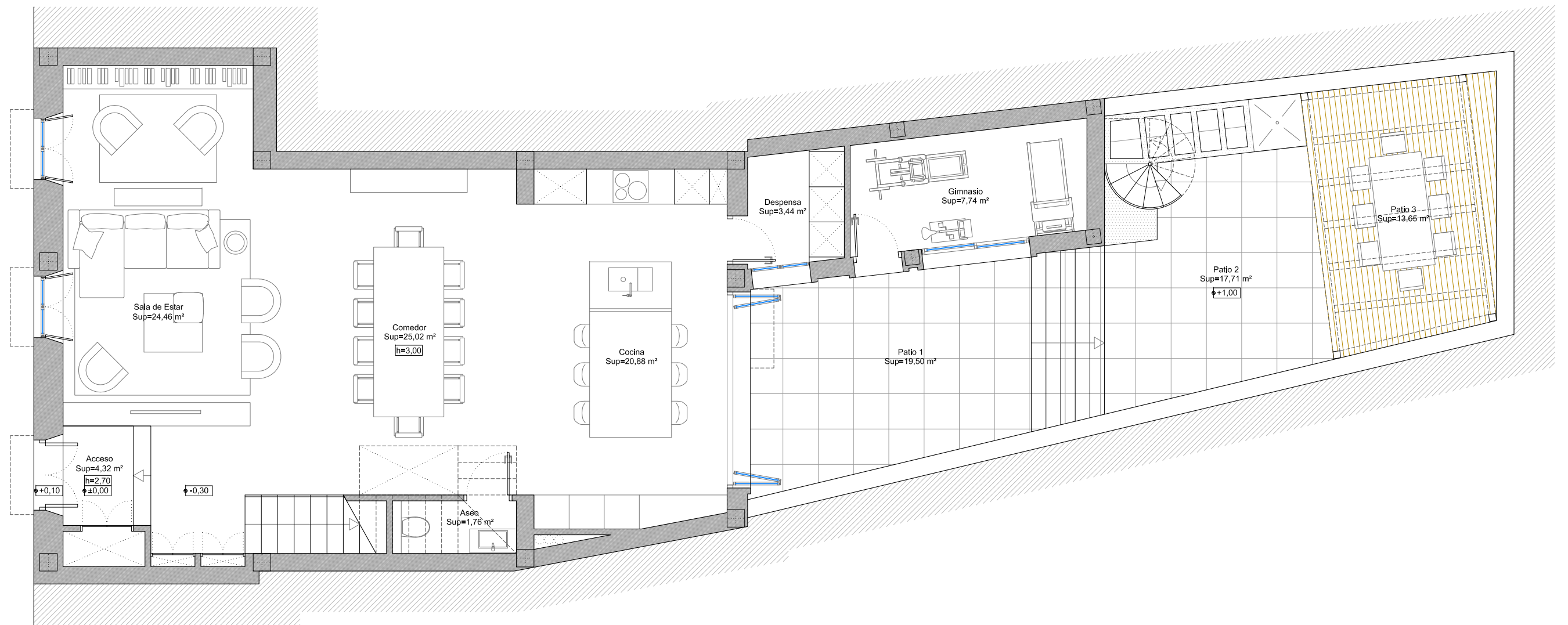
GROUND FLOOR
