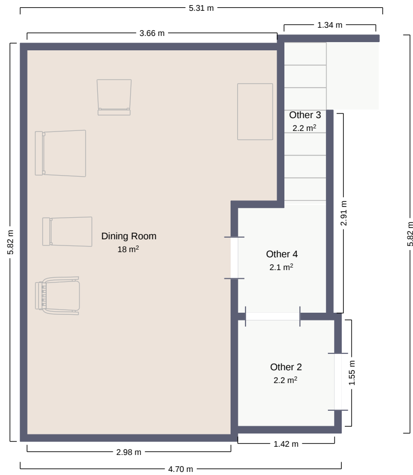
Floor 1
