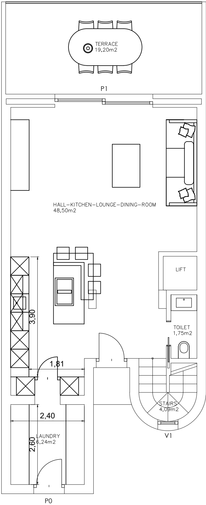
GROUND FLOOR - S.C.= 97.13 M2
