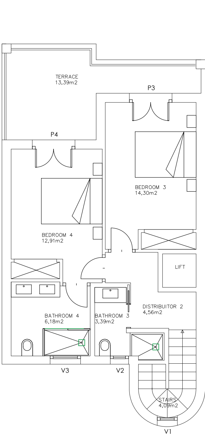
SECOND FLOOR - S.C.= 72.20 M2
