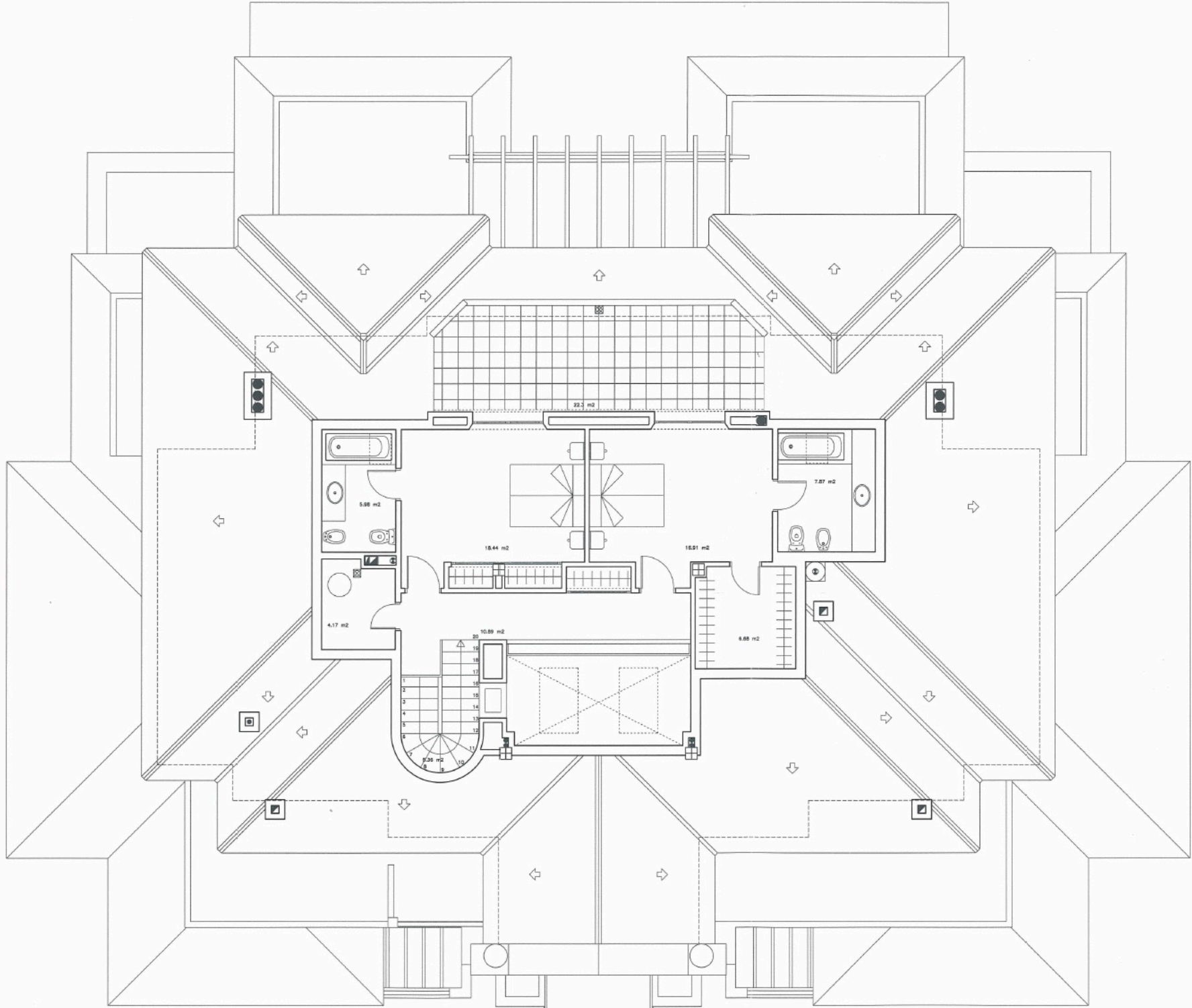
PLANTA ÁTICO (ALTA DÚPLEX) PENTHOUSE DUPLEX (UPPER FLOOR) E:1/100
