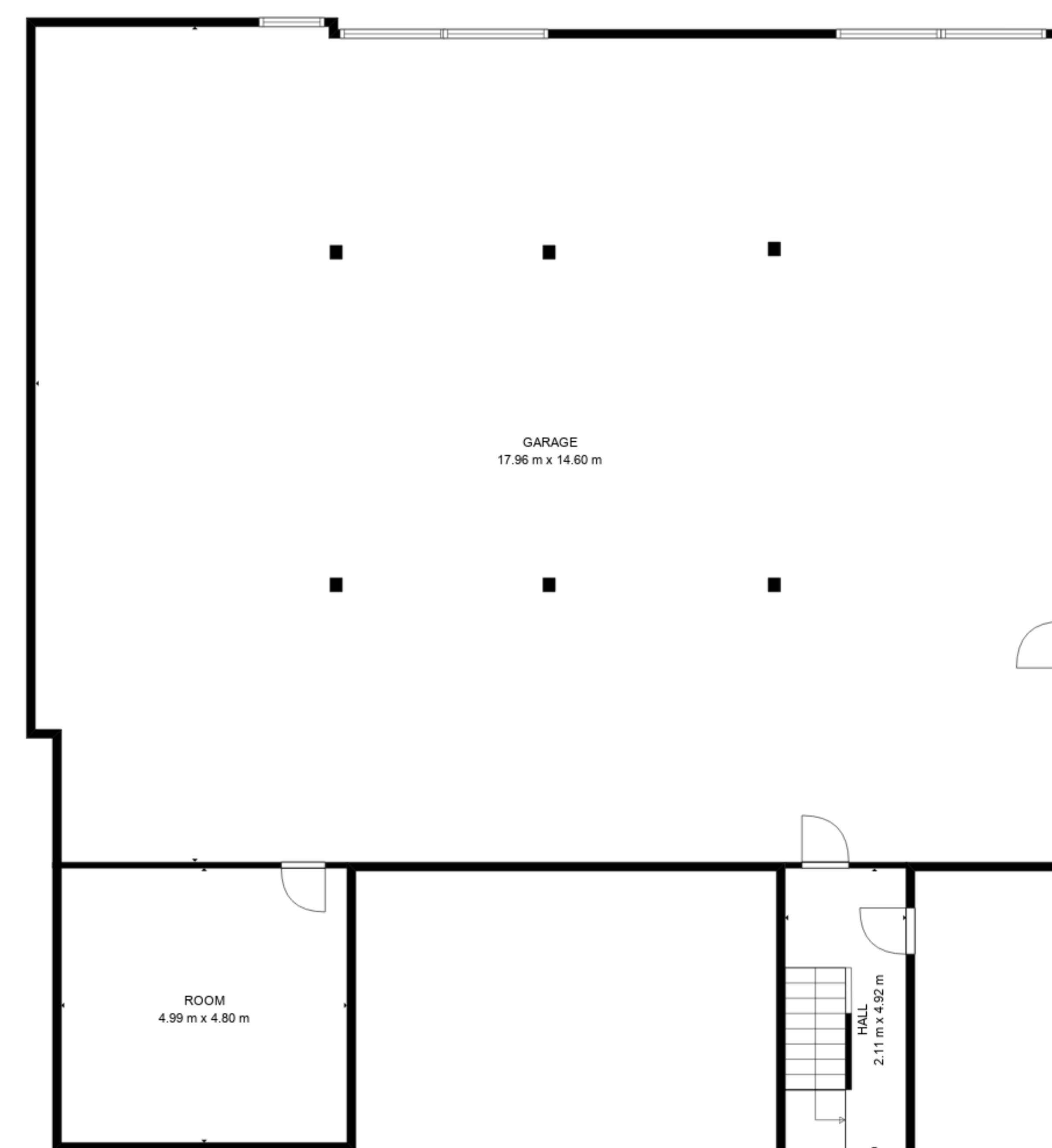
FLOOR 1
