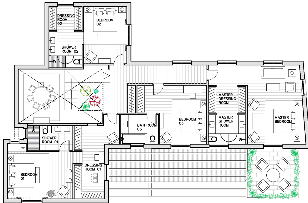
FIRST FLOOR
