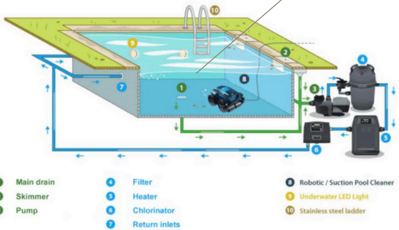
SALINE - CHLORINE WATER SYSTEM POOL
